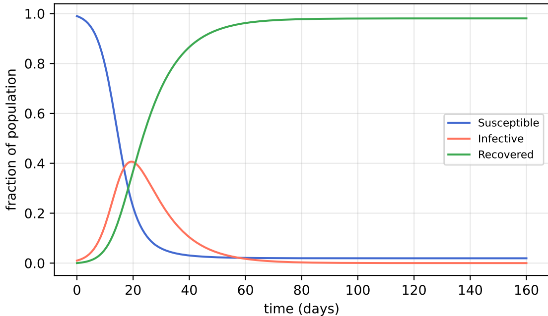
SIR epidemic curve
