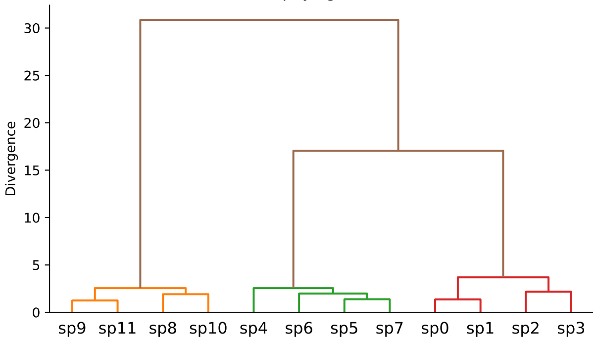
Rooted phylogenetic tree
