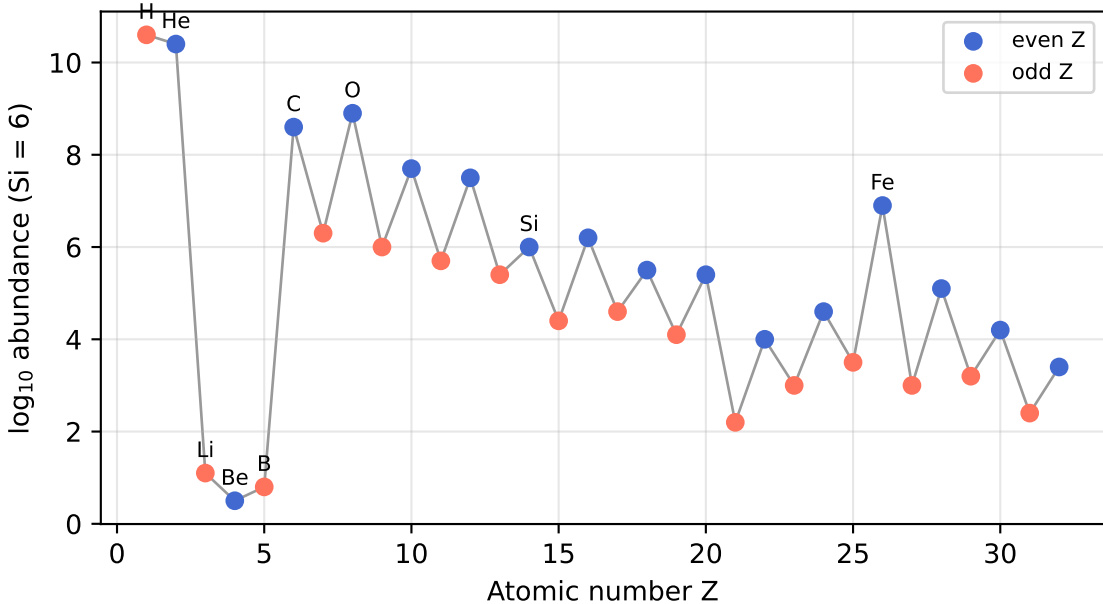
Oddo-Harkins sawtooth
