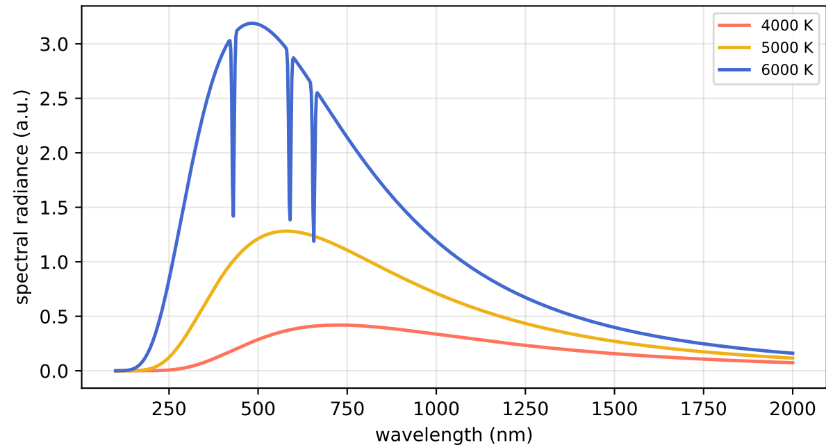
Blackbody continuum with absorption lines
