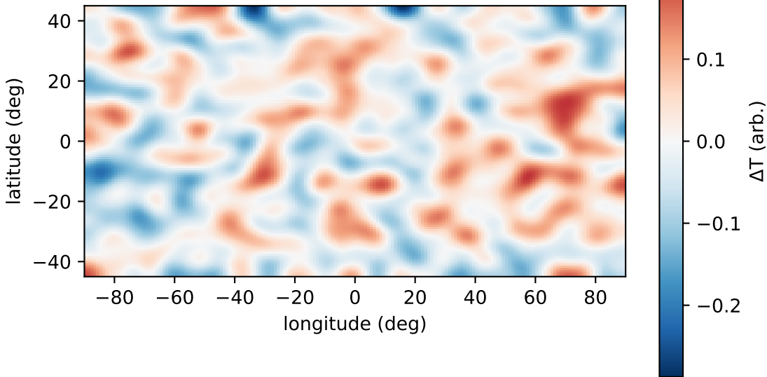
CMB temperature map (sky patch)
