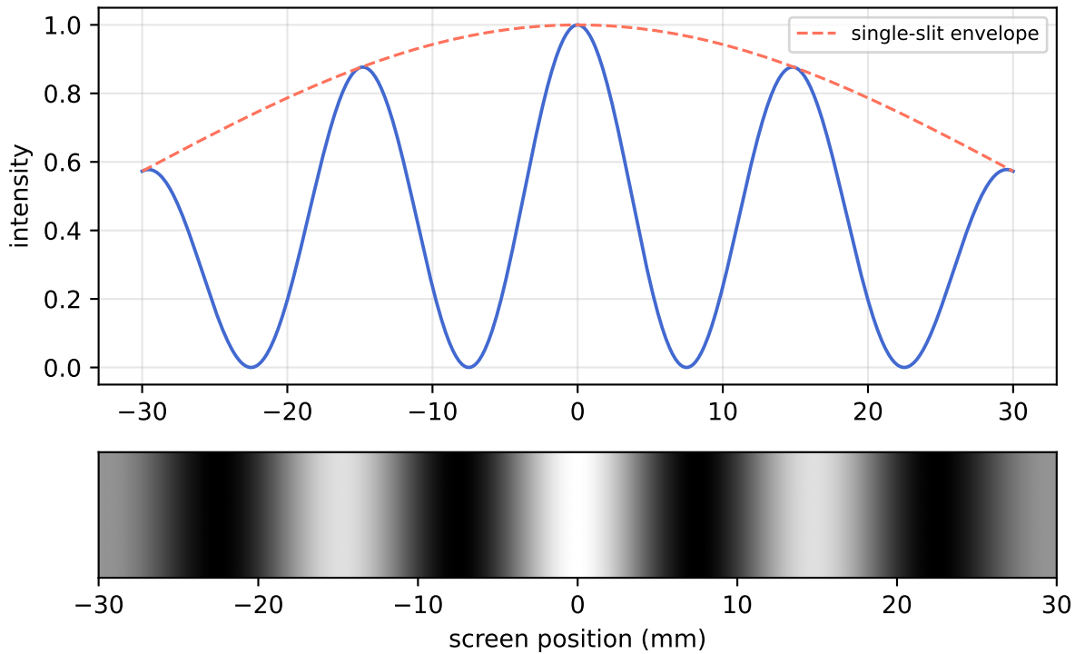
Two-slit interference
