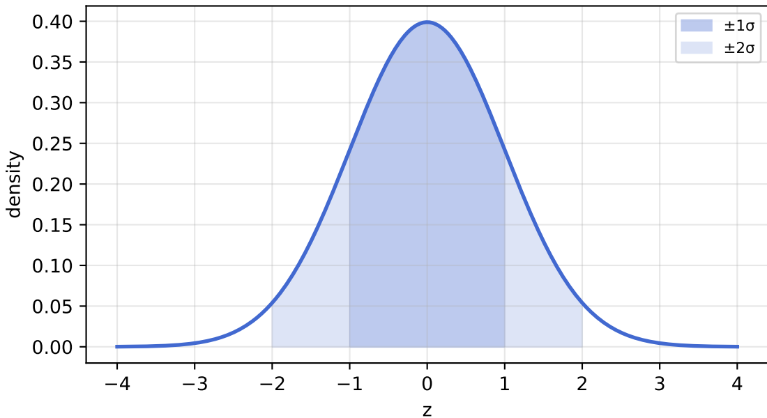
Standard normal distribution
