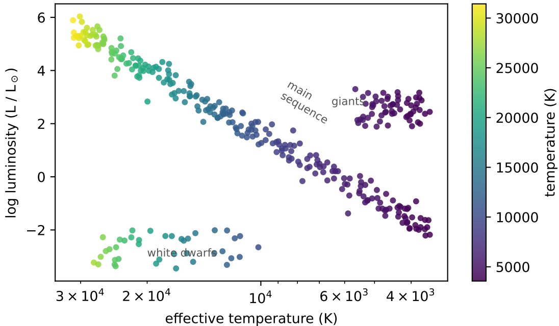
Hertzsprung–Russell diagram
