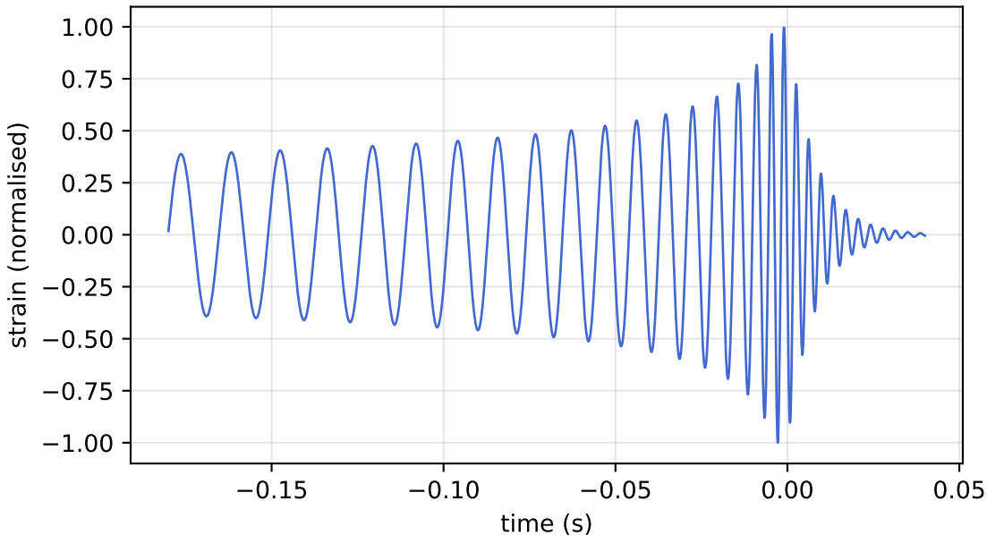
Gravitational-wave chirp (GW150914)
