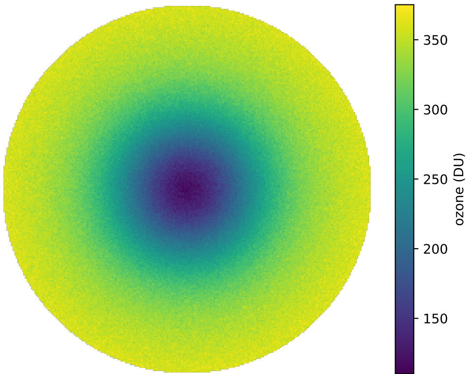
Ozone hole (total column)
