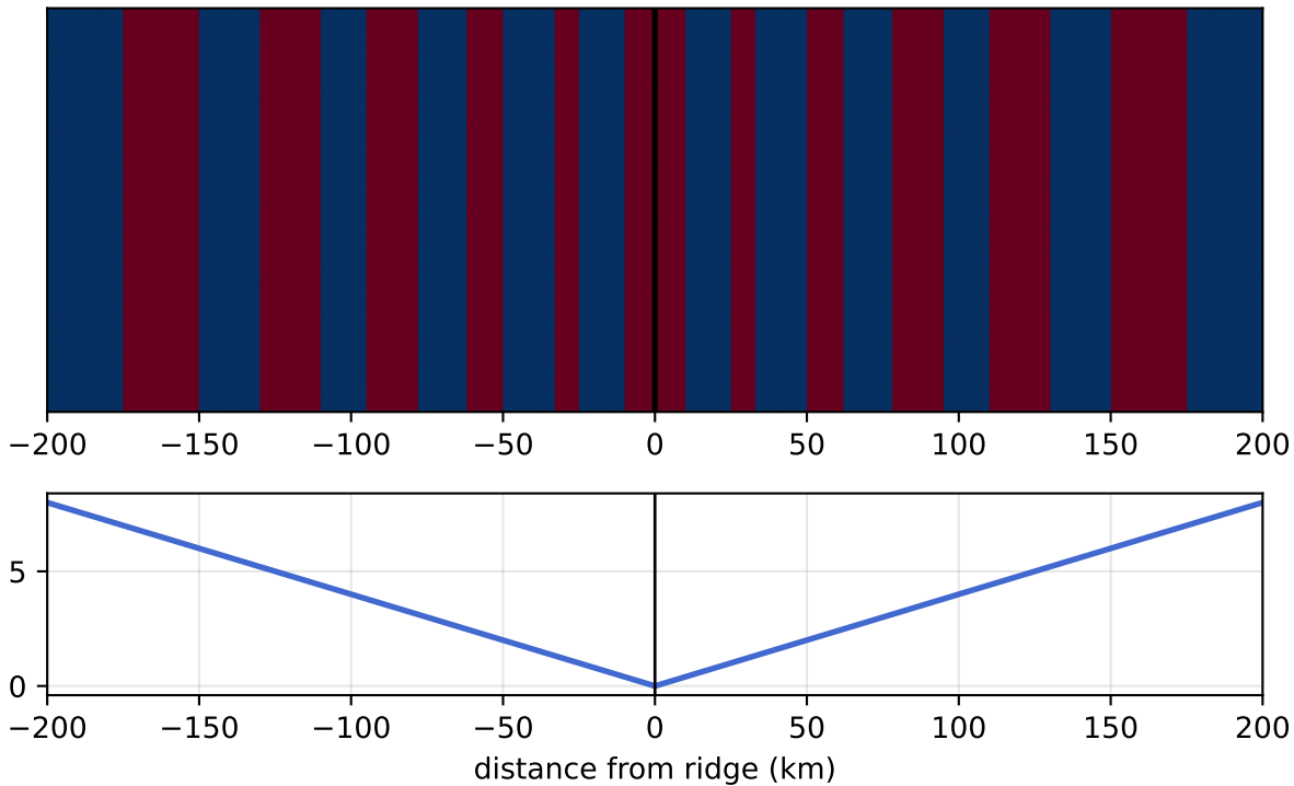
Symmetric magnetic anomaly stripes
