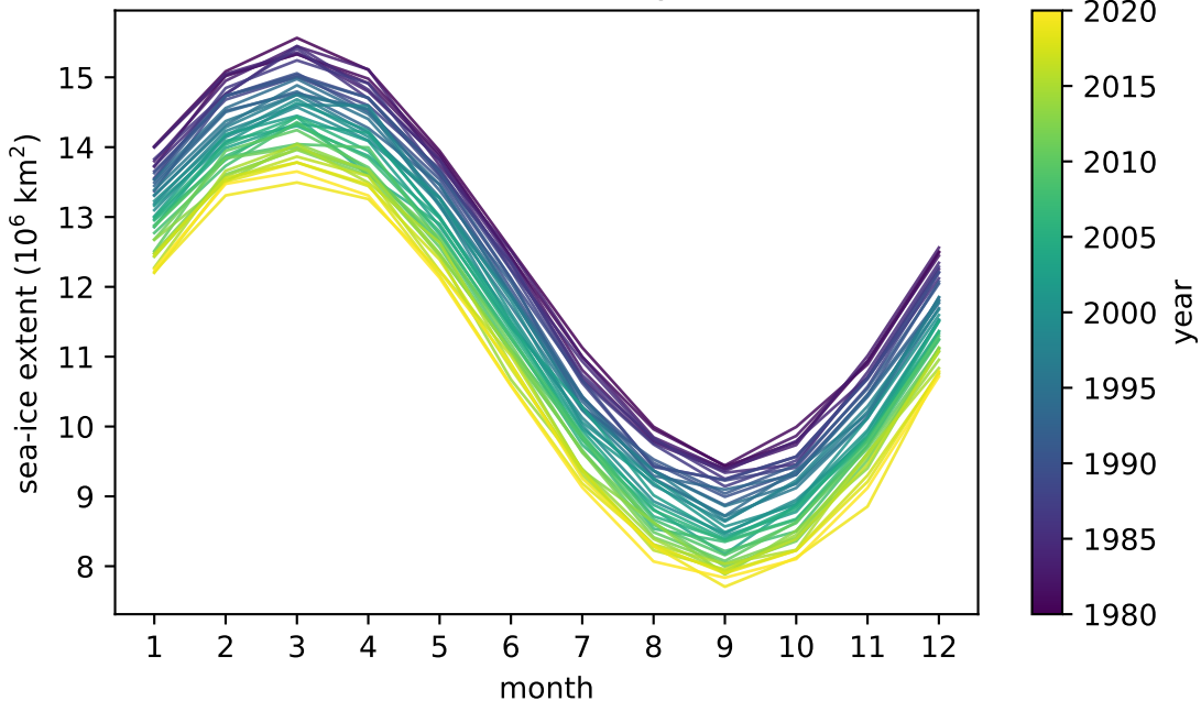
Sea-ice annual cycle
