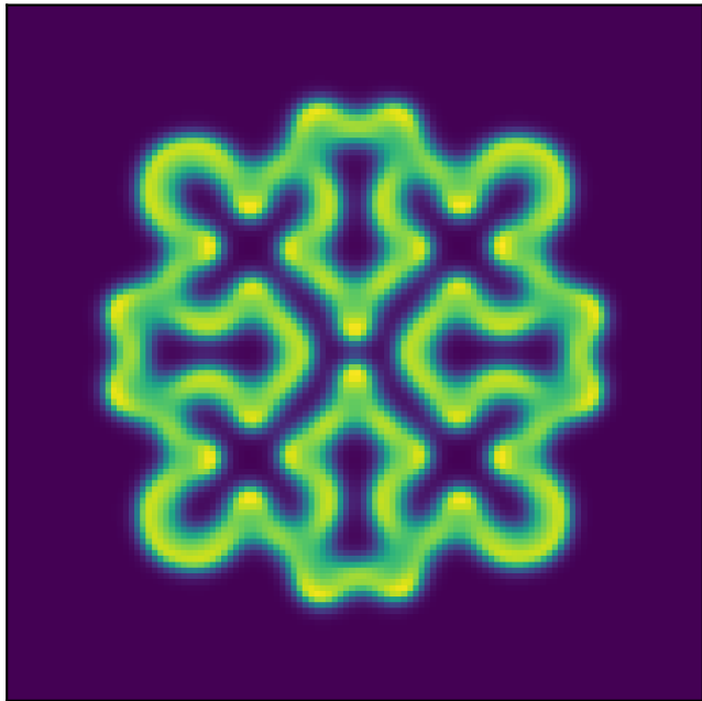
Reaction-diffusion (Turing) pattern
