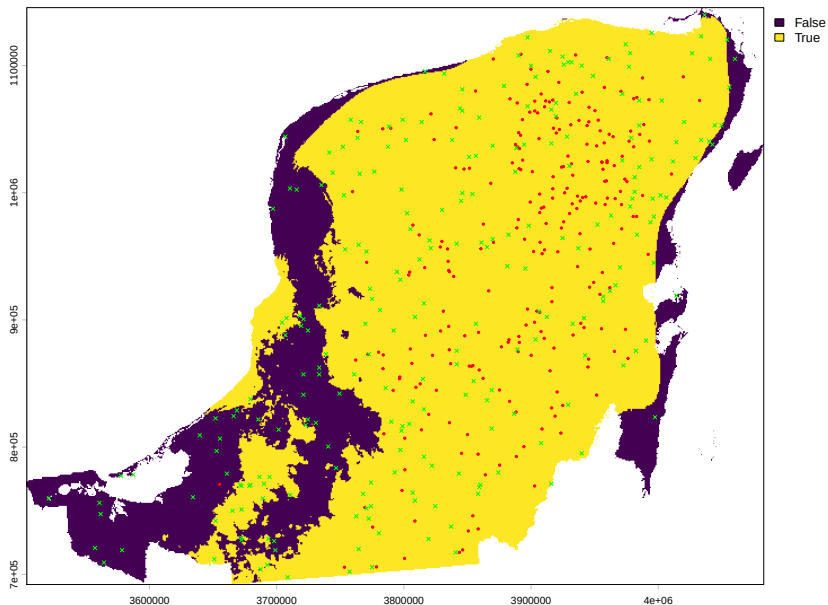
Fig. 2.6. Result of recursive thresholding with a threshold of 0.60.
