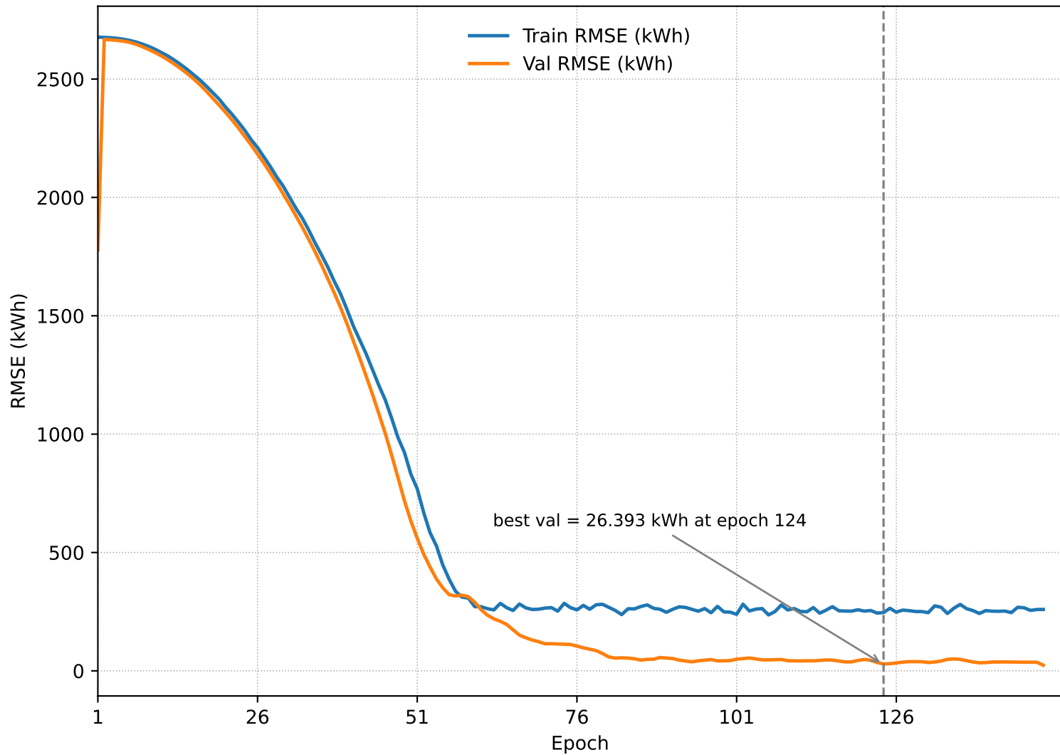
Training & Validation RMSE (kWh)
