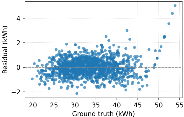
Residuals vs. truth
