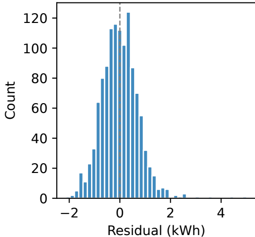
Residuals histogram
