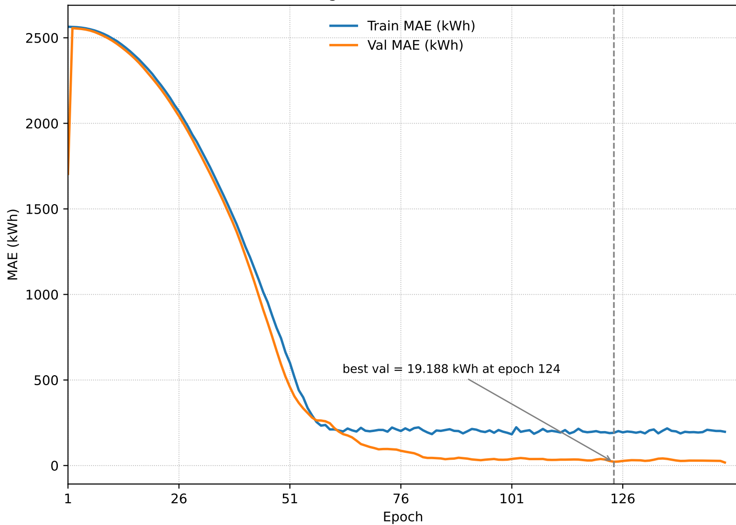
Training & Validation MAE (kWh)
