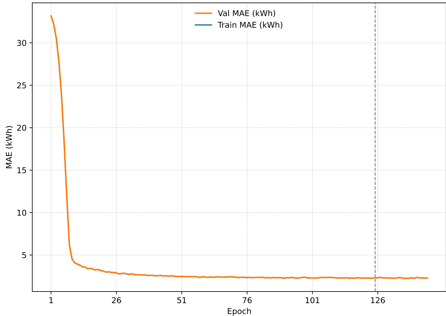
Training & Validation MAE (kWh)
