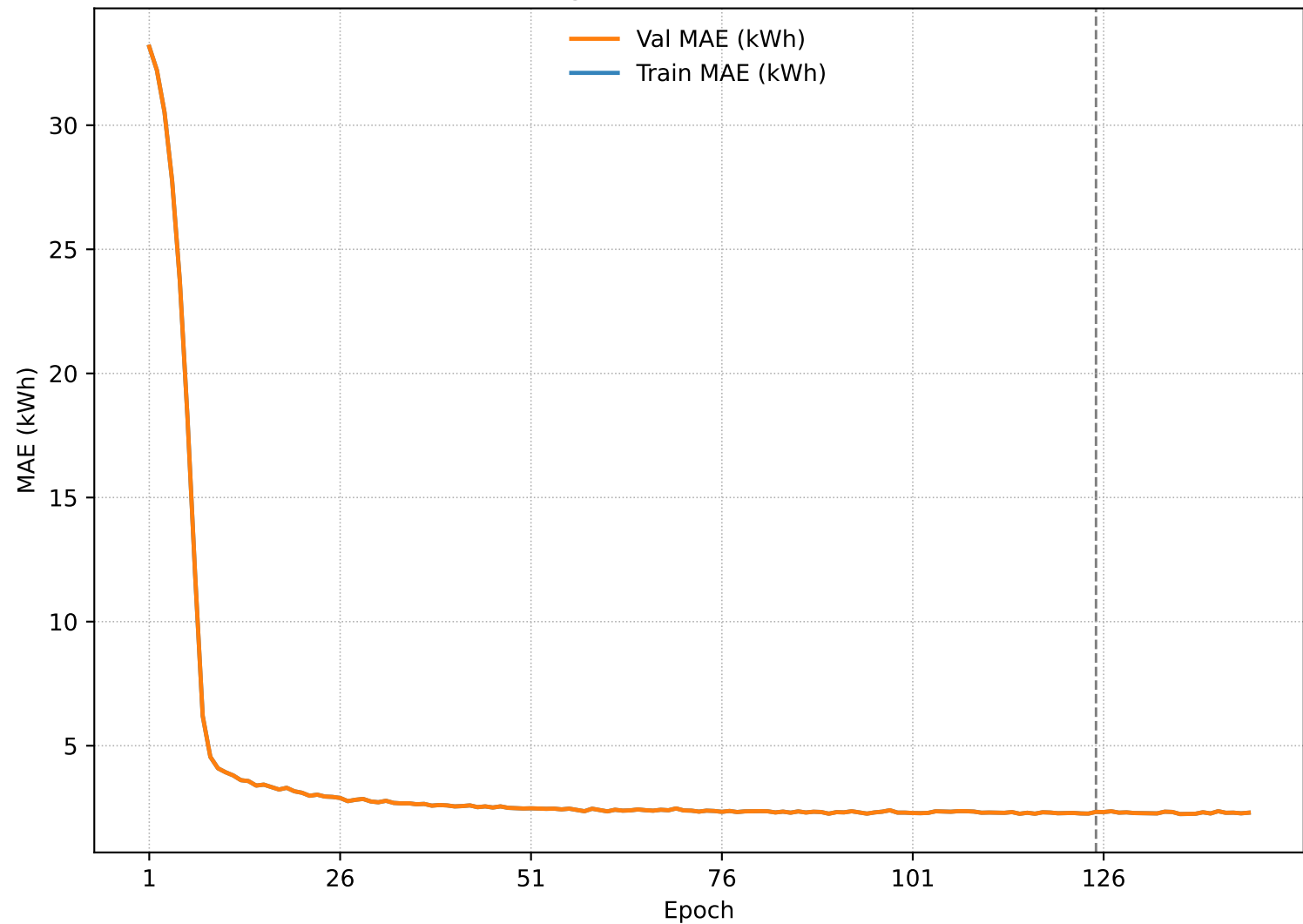
Training & Validation Loss (MAE)
