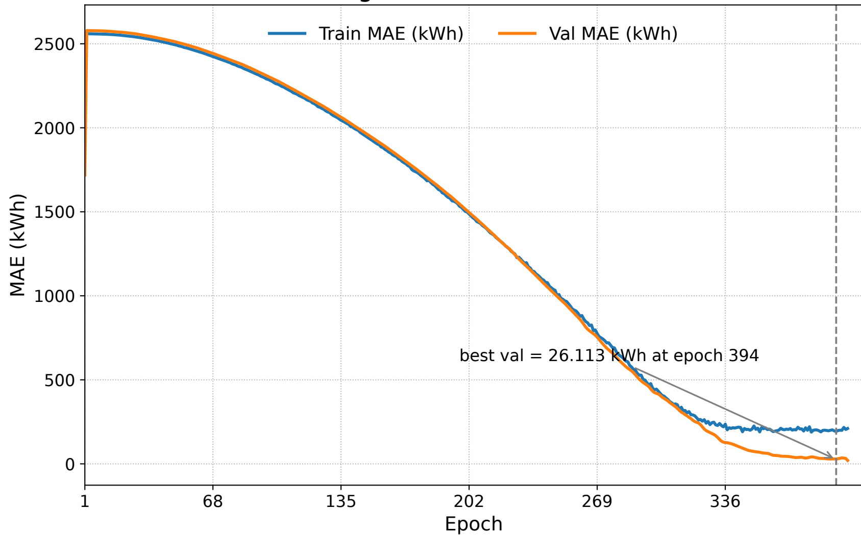
Training & Validation MAE (kWh)
