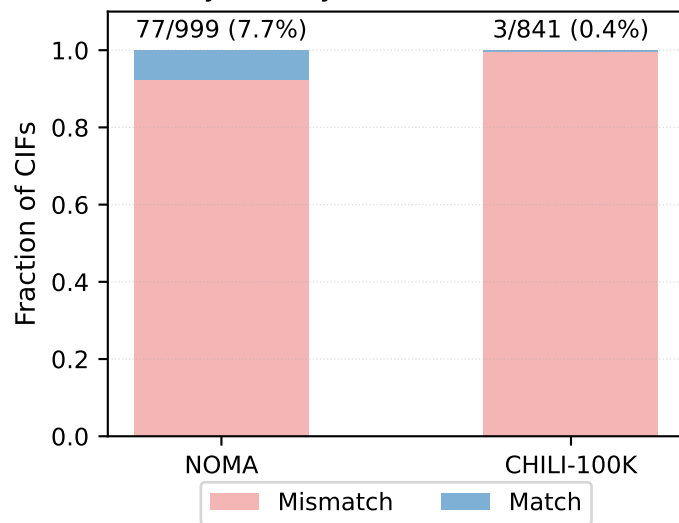
Symmetry-aware match rate
