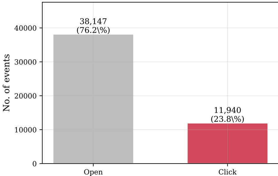
Distribution of the target variable
