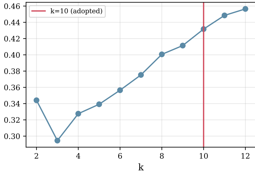
Mean silhouette
