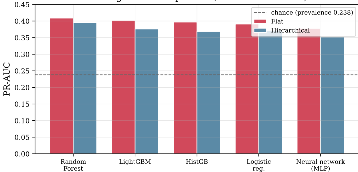
M2: algorithm comparison (flat vs hierarchical)
