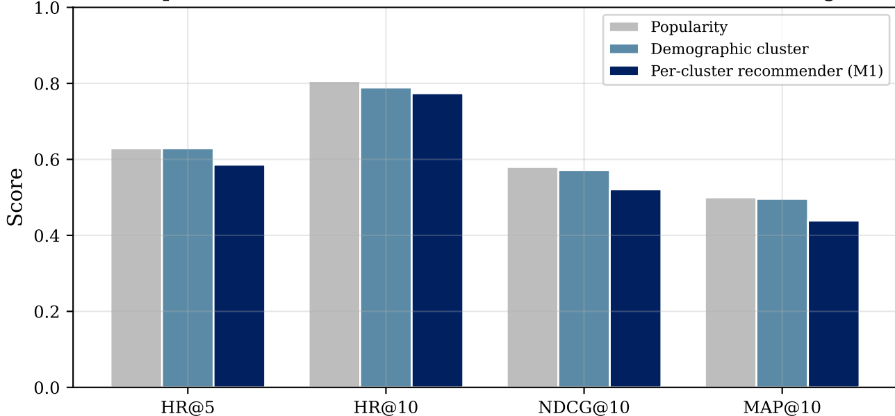
M3: per-cluster recommender (M1) vs baselines (test, no leakage)
