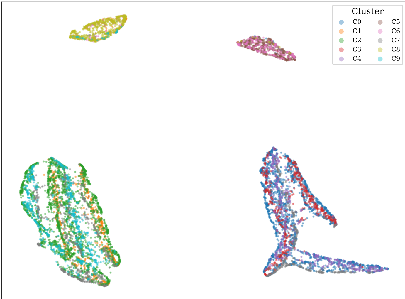
UMAP projection of the 10 demographic clusters (M0) n = 10,000 users, 4D latent \rightarrow 2D UMAP
