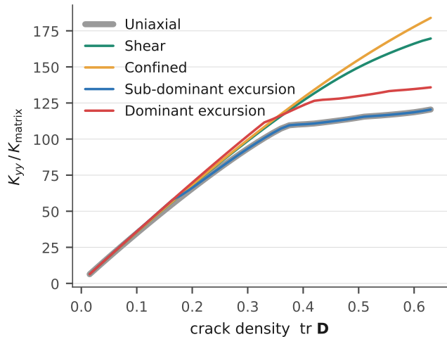
(b) effective permeability, five loading paths
