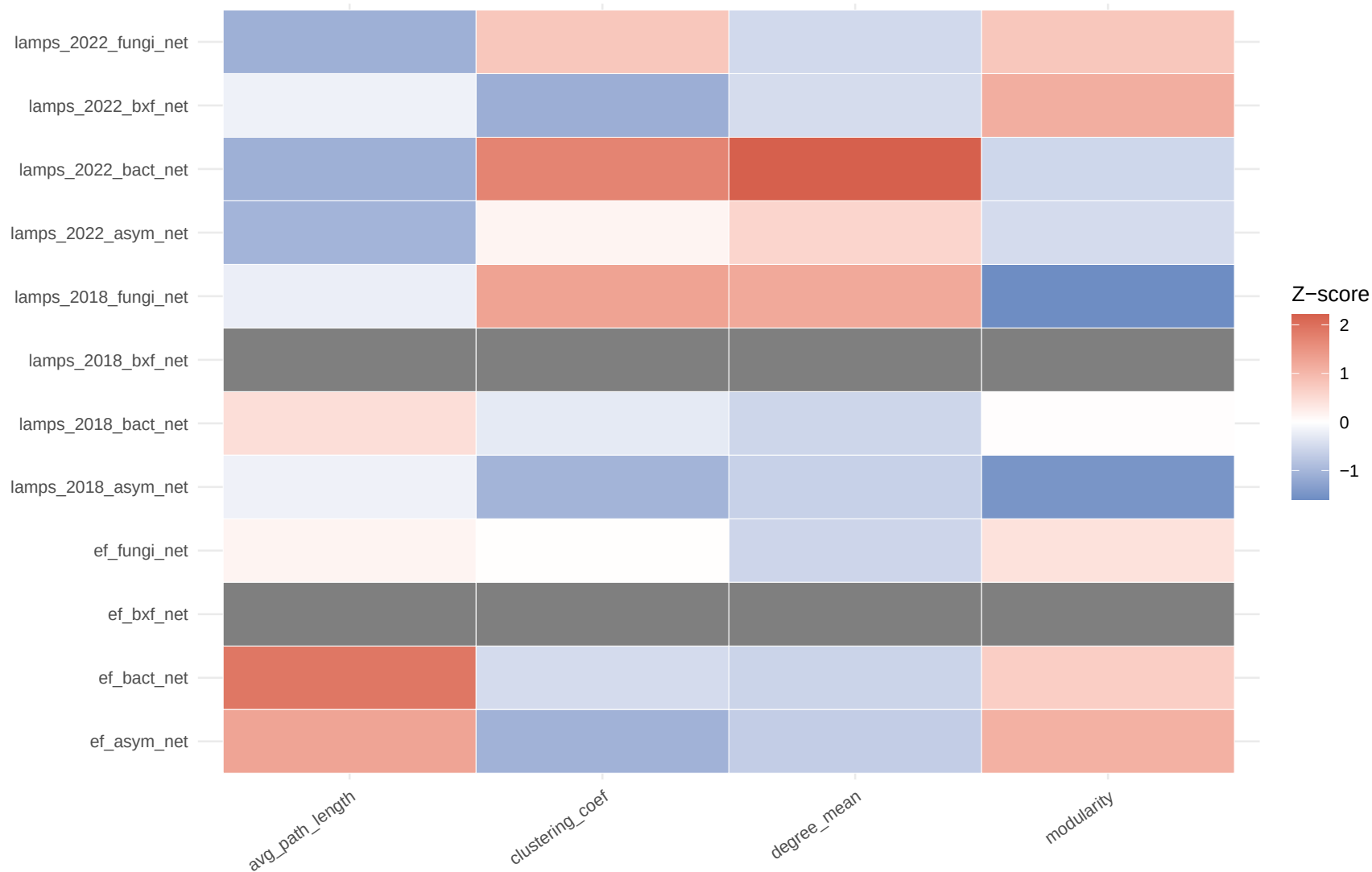
Network topological properties (z-scored)
