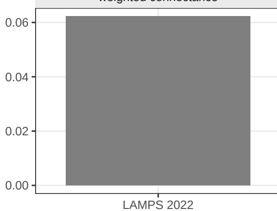
weighted connectance
