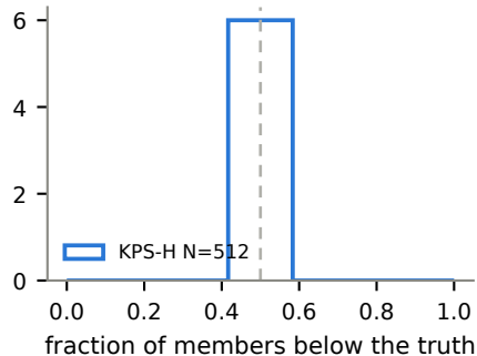
Navier-Stokes
