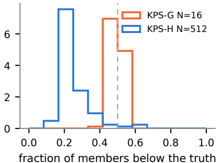
Inverse scattering
