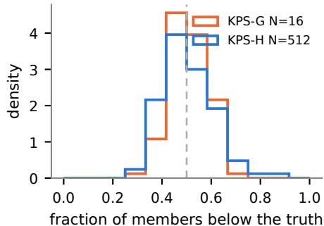
Black-hole imaging
