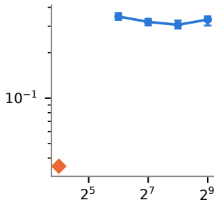
Inverse scattering
