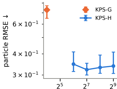
Black-hole imaging
