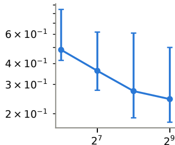
Navier-Stokes
