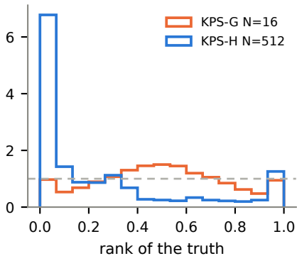
Inverse scattering
