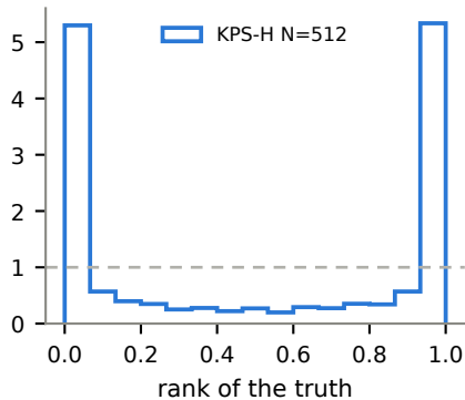
Navier-Stokes
