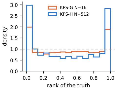
Black-hole imaging
