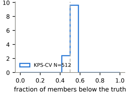
Navier-Stokes
