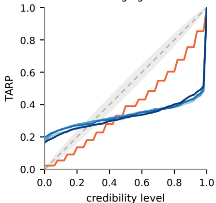
Navier-Stokes
