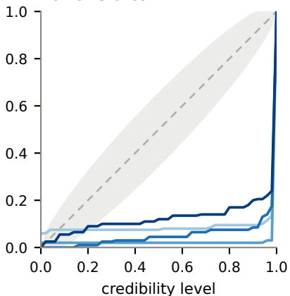
Navier-Stokes
