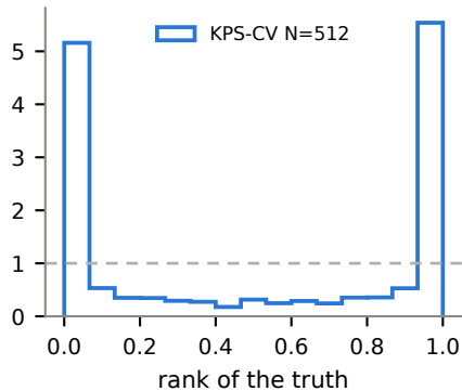
Navier-Stokes
