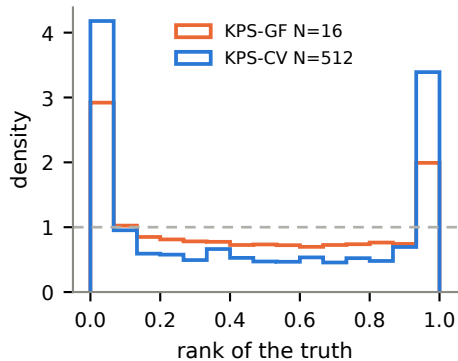
Black-hole imaging
