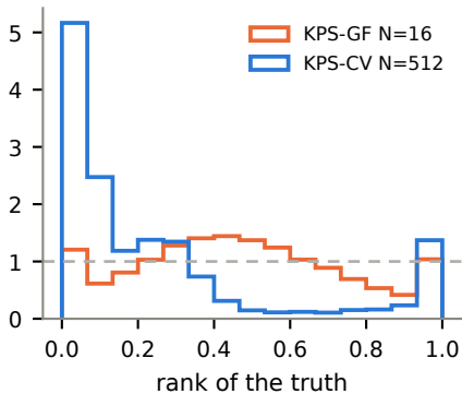
Inverse scattering
