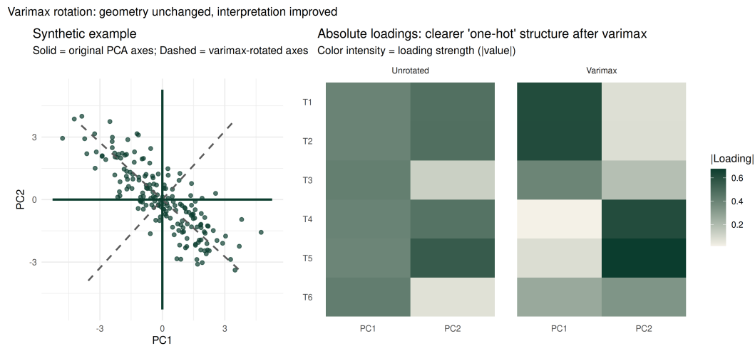
Figure 19: Synthetic illustration of varimax rotation. Left: identical point cloud with original (solid) and rotated (dashed) axes. Right: absolute loadings showing clearer, more concentrated structure after varimax.
