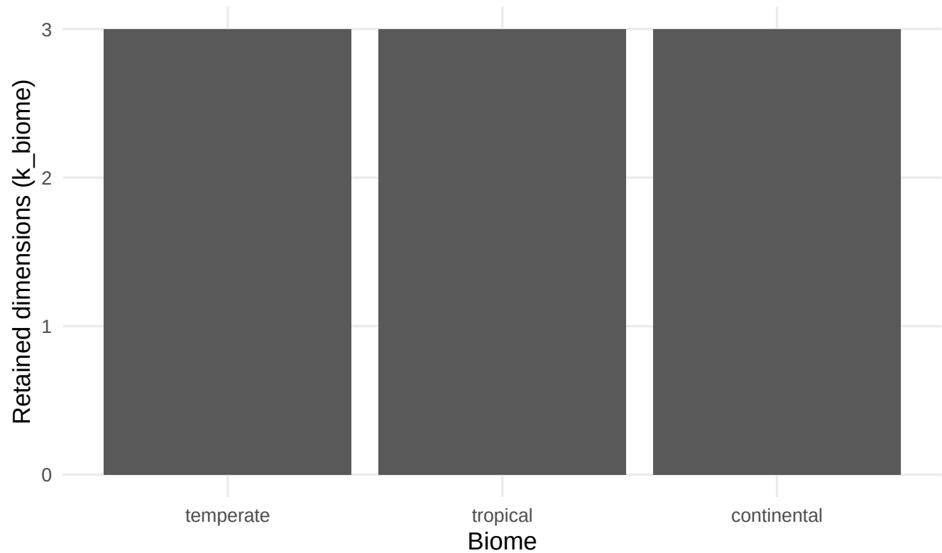
Retained PCA dimensionality per biome (paran)
