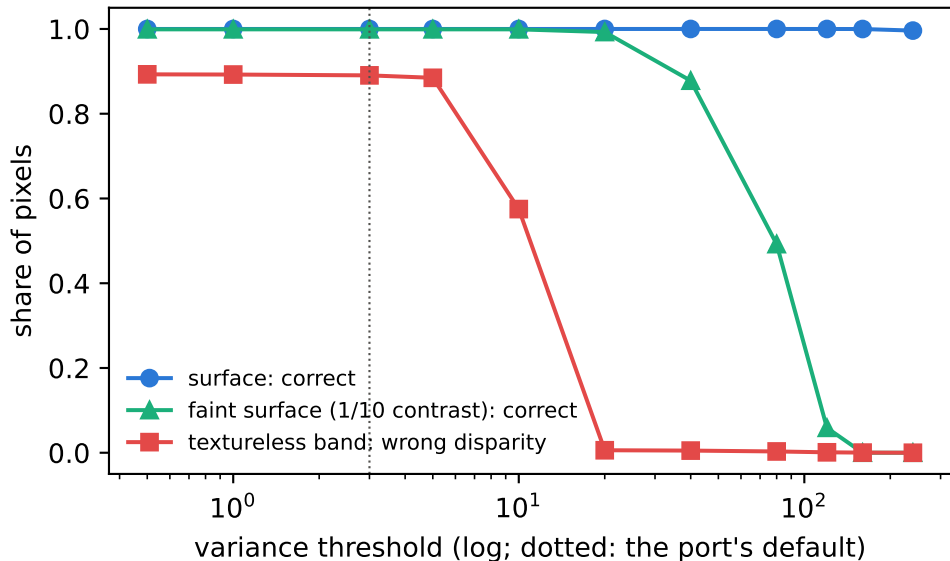
Abb. 5.32: the variance threshold
