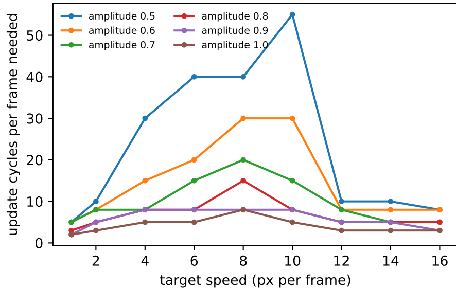
Abb. 6.9: tracking (dissertation parameters)
