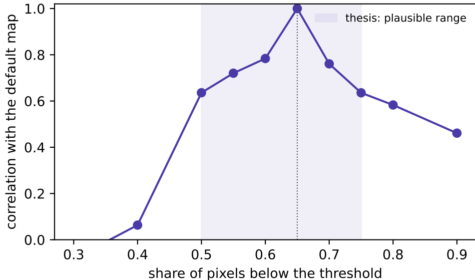
Abb. 5.15: region-growing threshold
