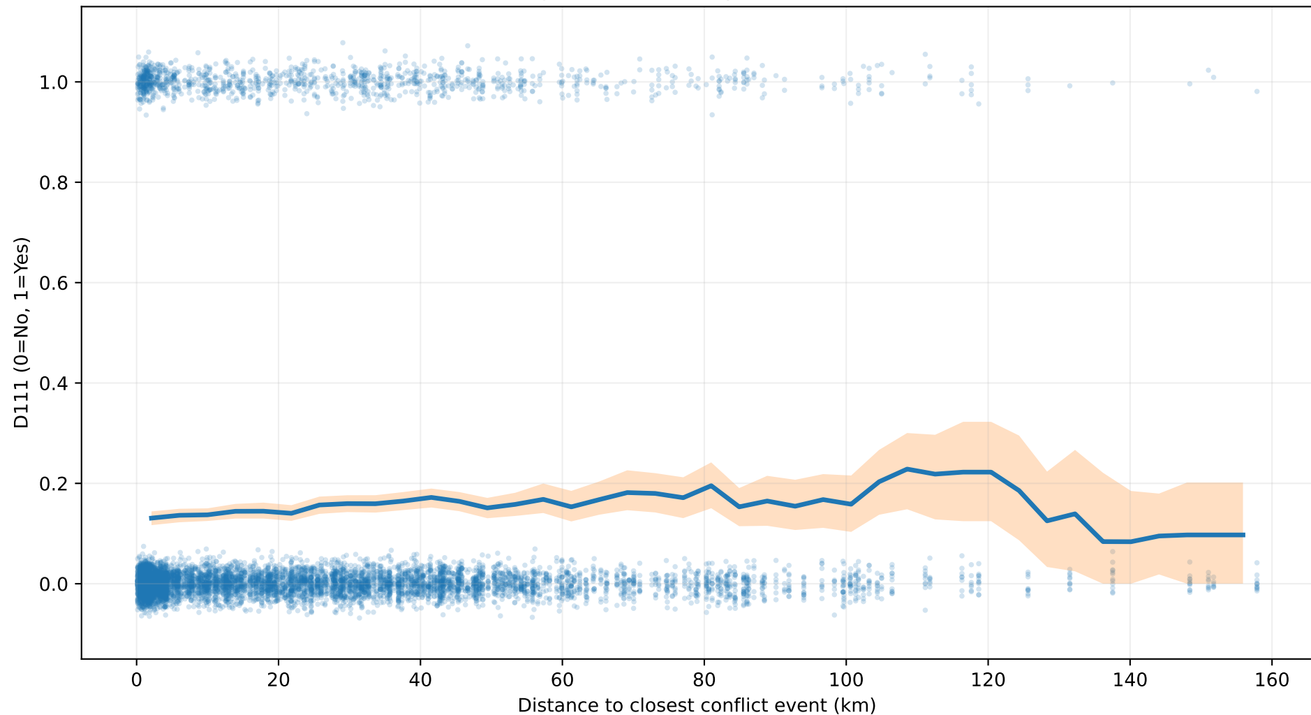
H9: IPV (D111) vs distance to closest conflict event Unweighted • Bootstrap 95% CI (n=500)
