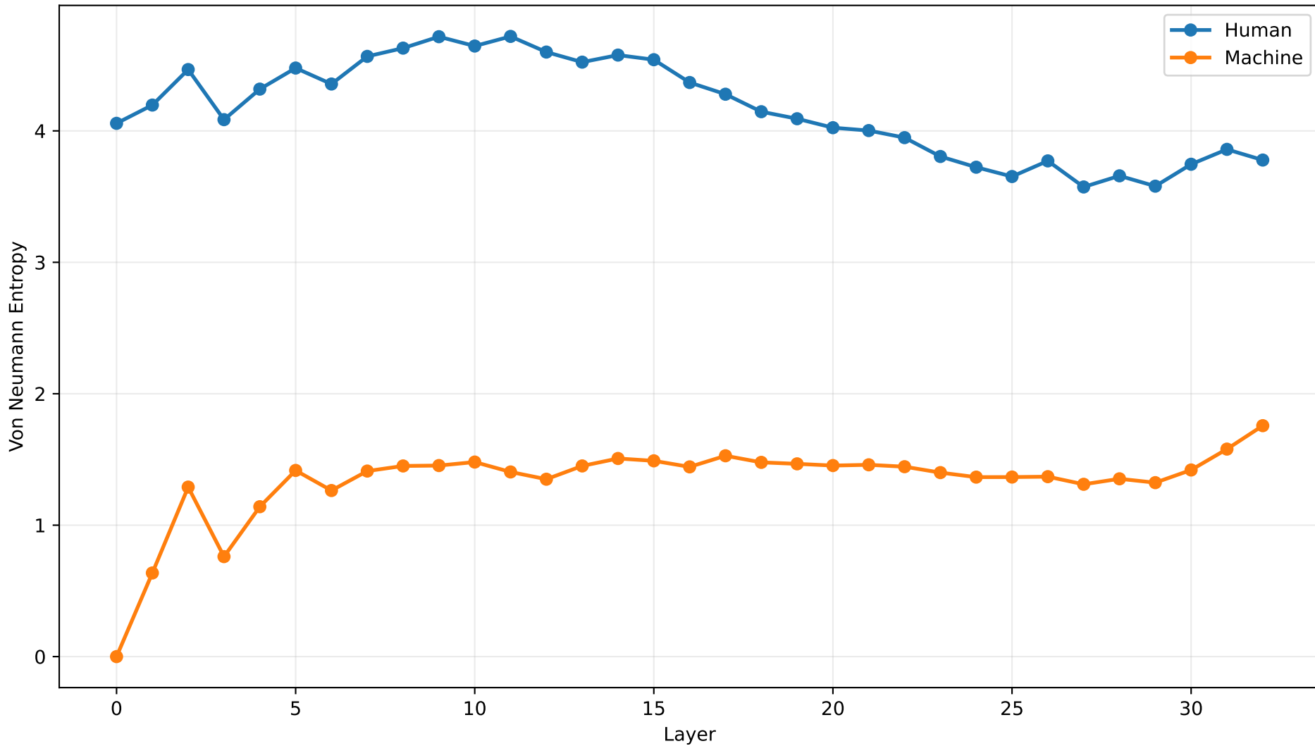
Von Neumann Entropy by Layer | d_m4_domains:wikipedia
