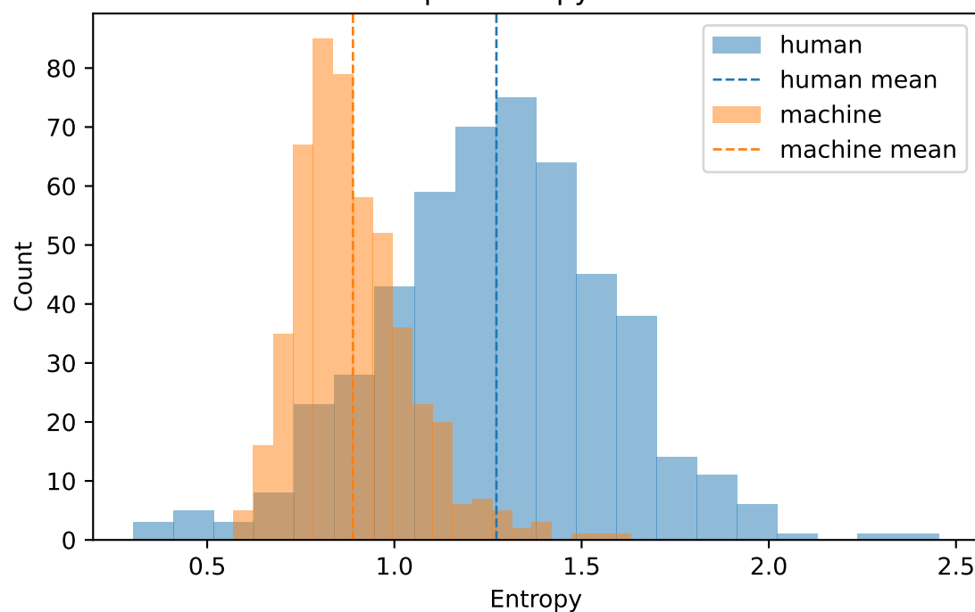
Vocab Entropy Change Mean
