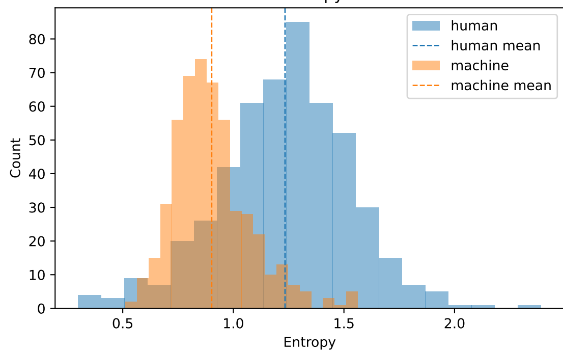
Entropy (Mean/Std/Change) by Label | N1000 | Model qwen_8b | Data wikipedia_chatgpt
