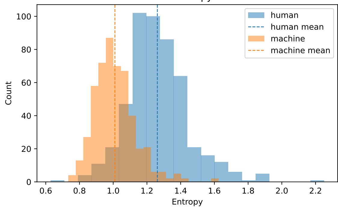
Entropy (Mean/Std/Change) by Label | N1000 | Model qwen_8b | Data wikipedia_chatgpt
