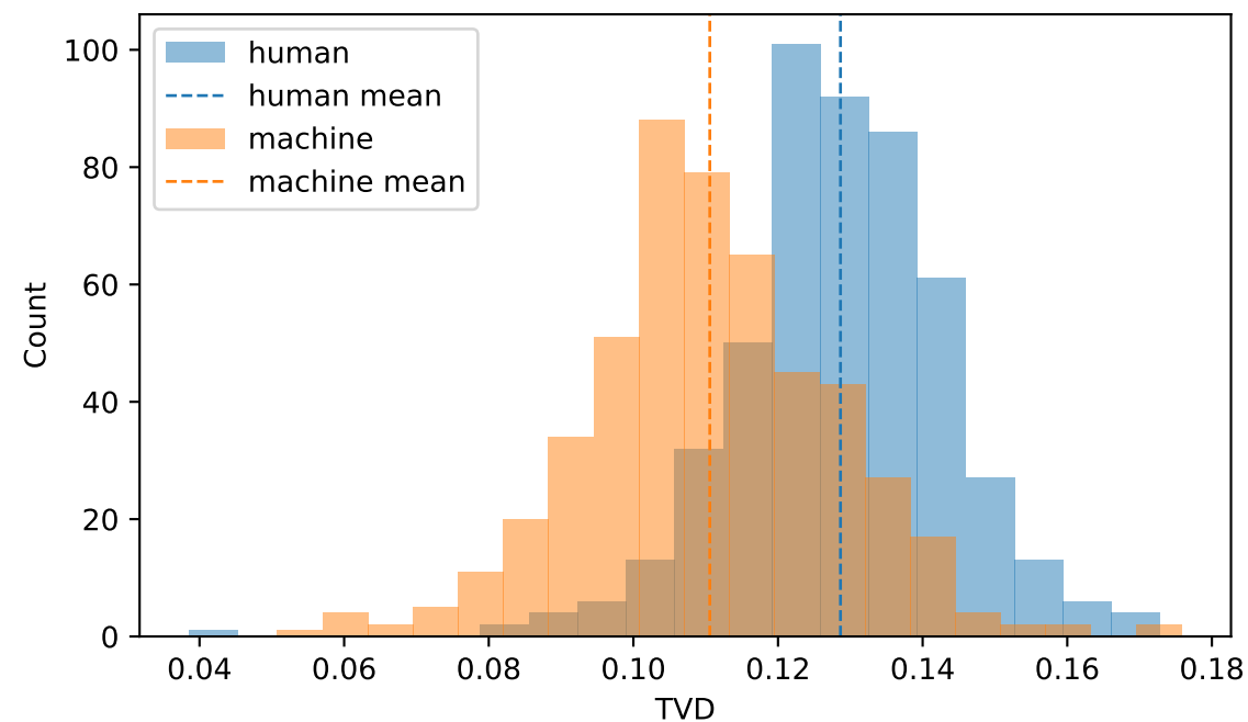
Top-K TVD Std
