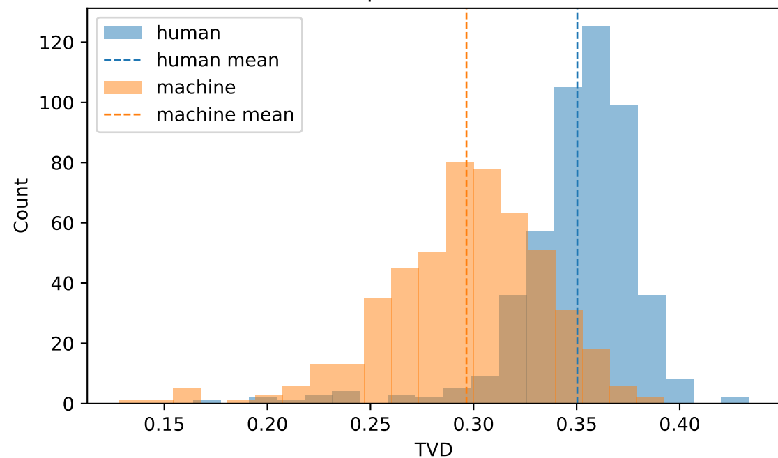
Top-K TVD Mean
