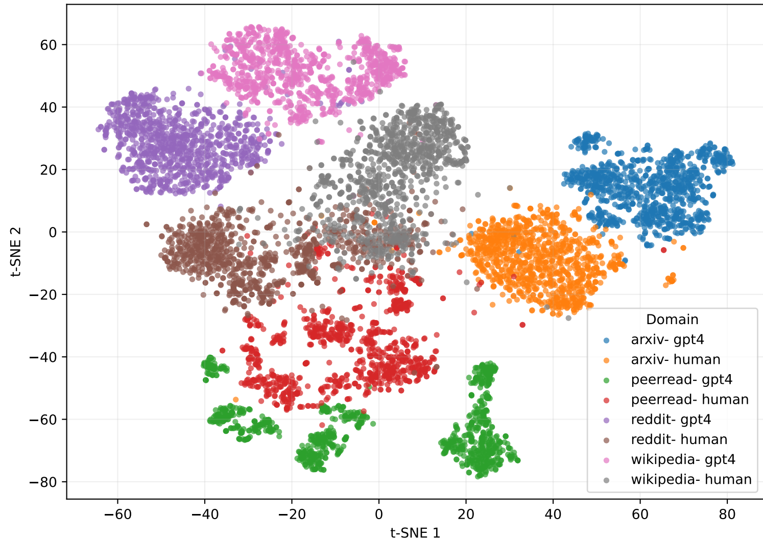
t-SNE of Middle-Layer Representations by Domain
