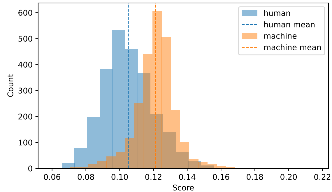
Magnitude Std
