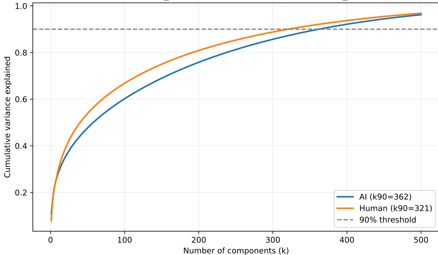
raidDomain_wiki: AI vs Human rank profile (llama_8b)
