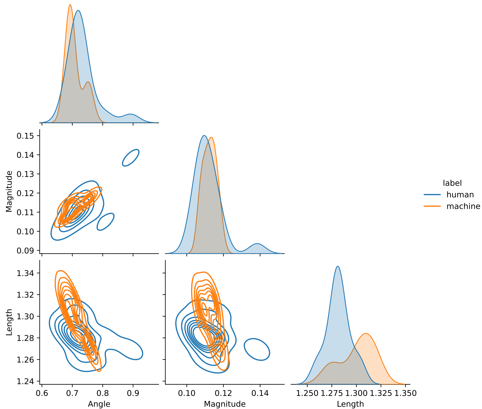
Pair Plot (Means) | N30 | Model qwen_06b | Data wikihow_chatgpt | LastToken 1 | DiffVec 1
