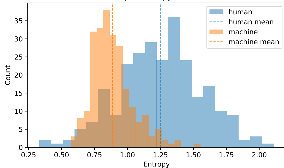
Top-K Entropy Mean
