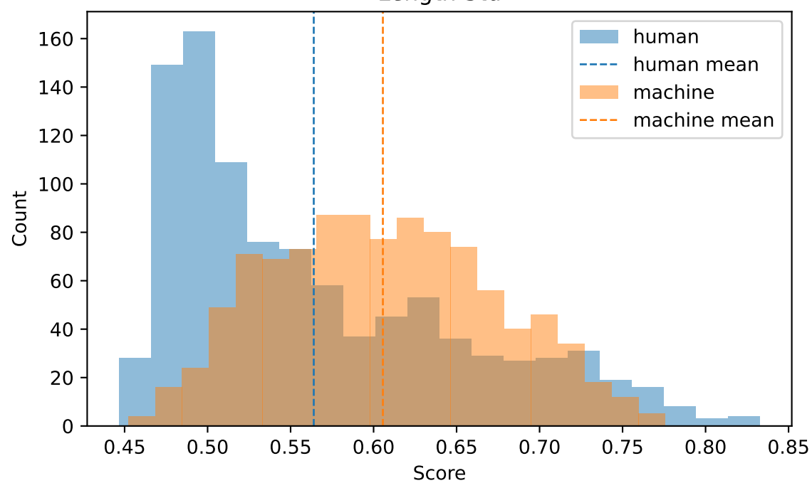
Length Std
