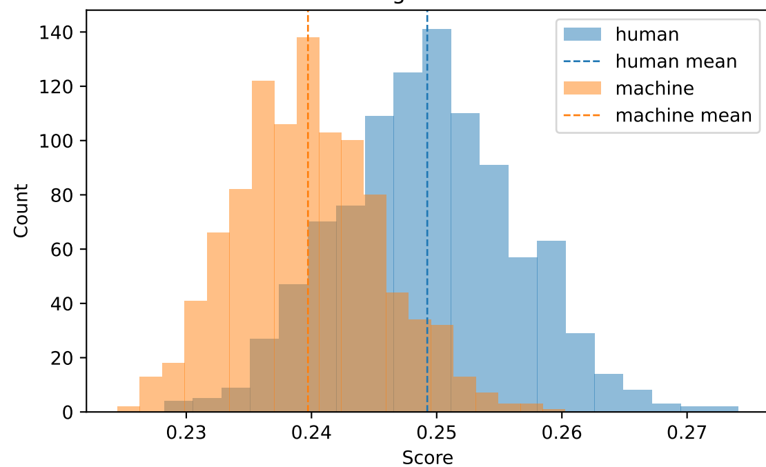
Magnitude Mean
