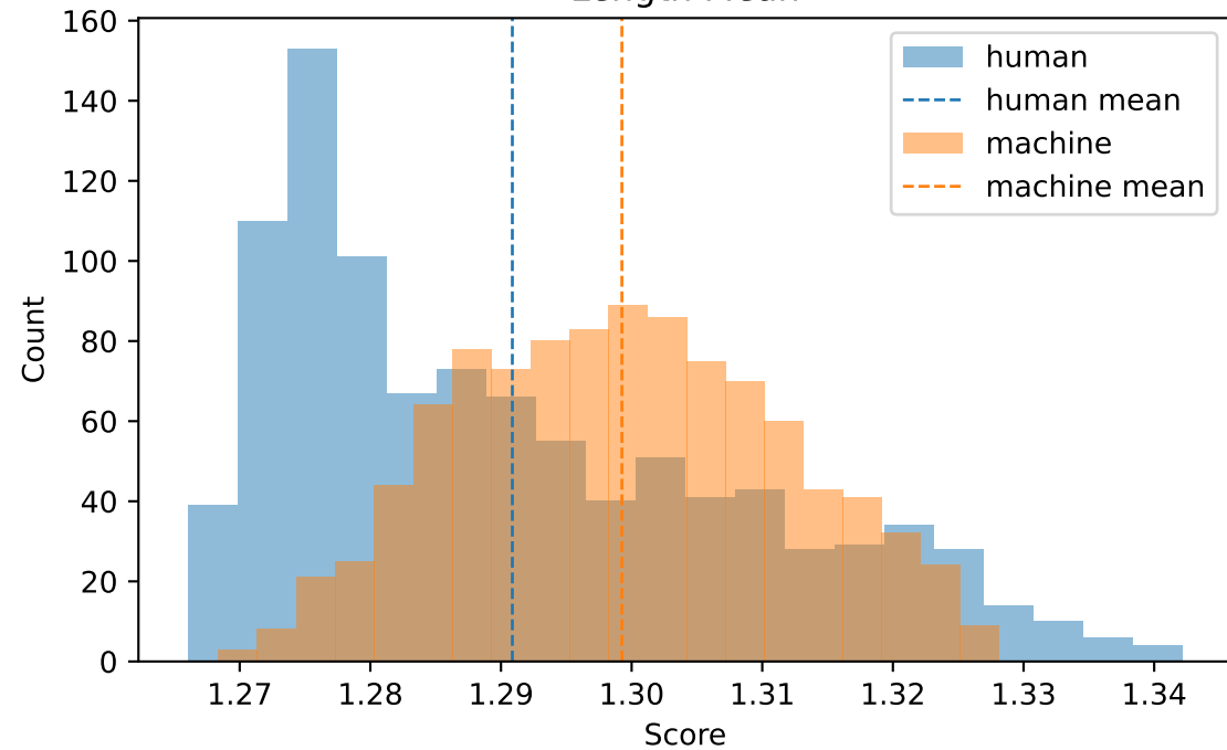
Length Mean
