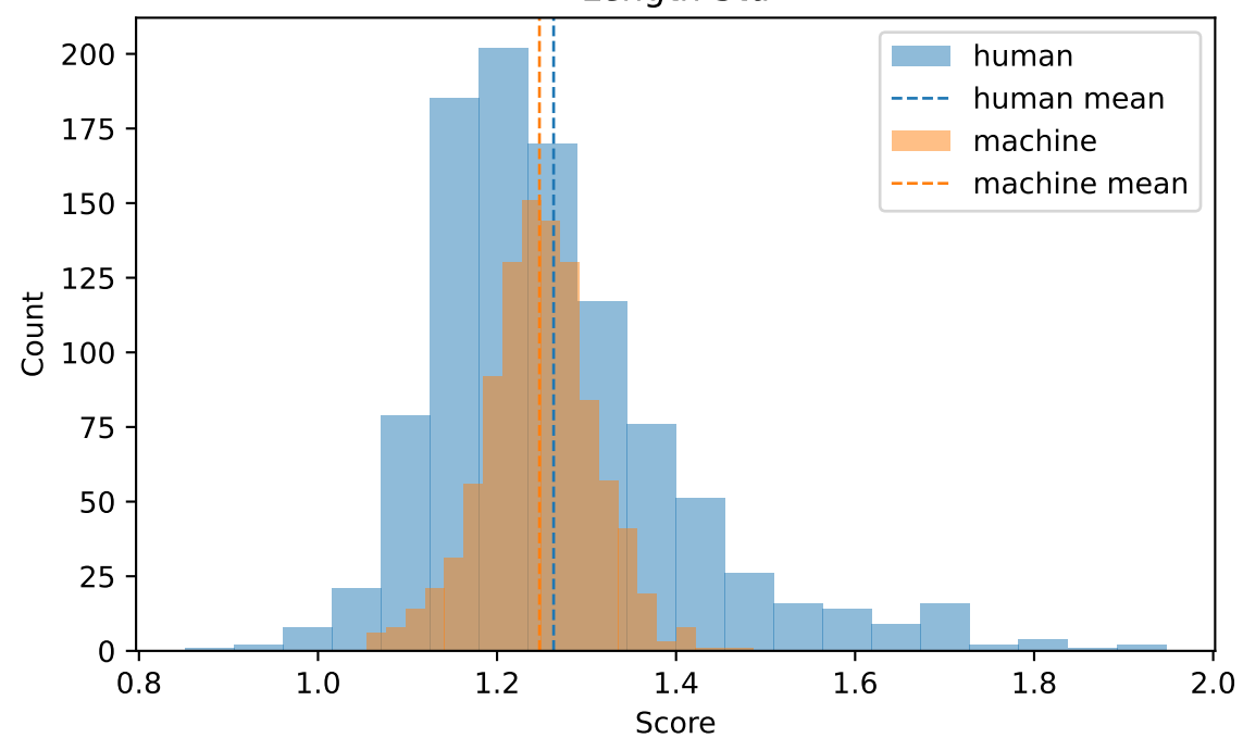
Length Std
