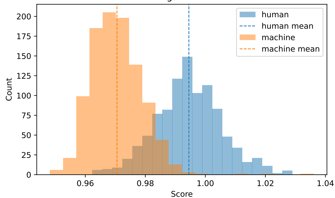
Magnitude Mean
