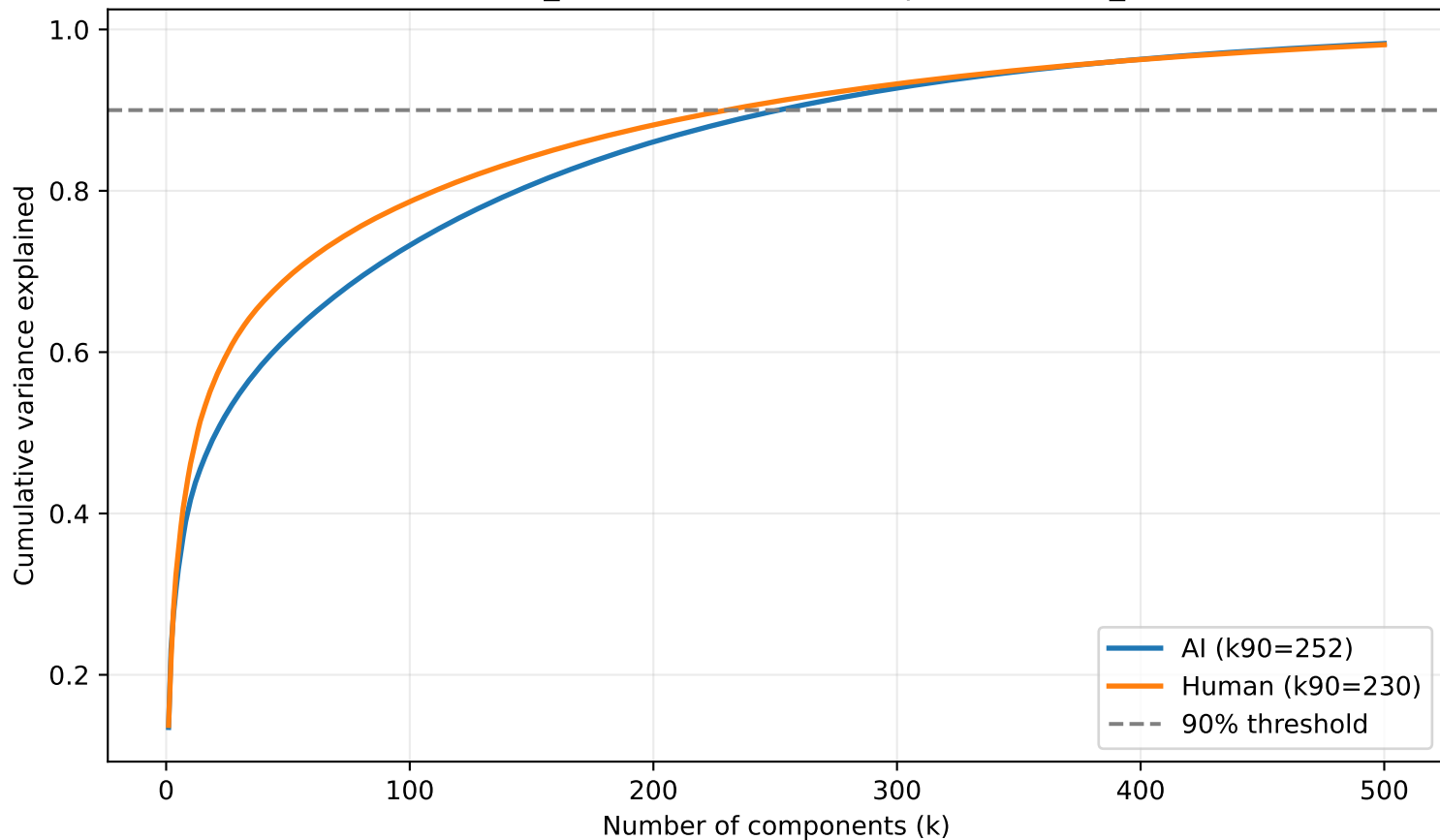
multisocial_de: AI vs Human rank profile (llama_8b)
