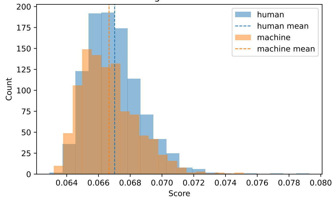
Length Mean
